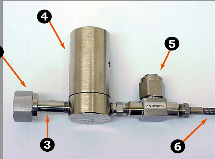
# 8784 LCO 2 Filter Housing ( ④ + ⑤ )
